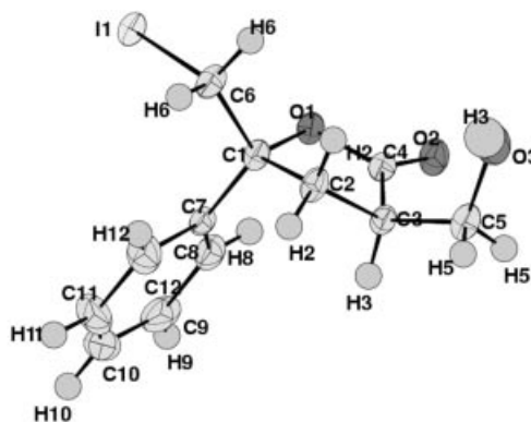
Figure 1. View of the crystal structure of 8a showing a cis relationship between the -\text{CH}_2\text{OH} and -\text{CH}_2\text{I} substituents; the ellipsoids represent atomic displacement parameters at the 50% probability level
