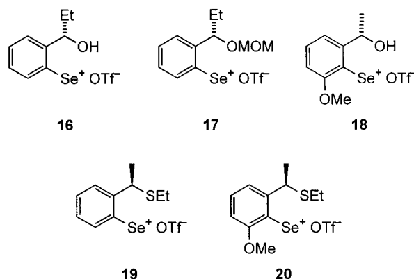
Figure 3. Chiral selenium electrophiles
